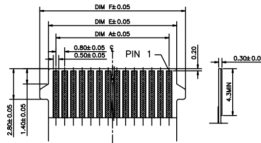
RECOMMENDED FPC/FFC DIMENSIONS
